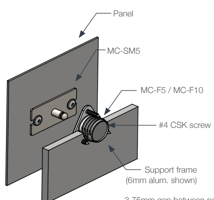
Cutaway exploded view (nts)
