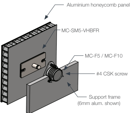
Cutaway exploded view (nts)
